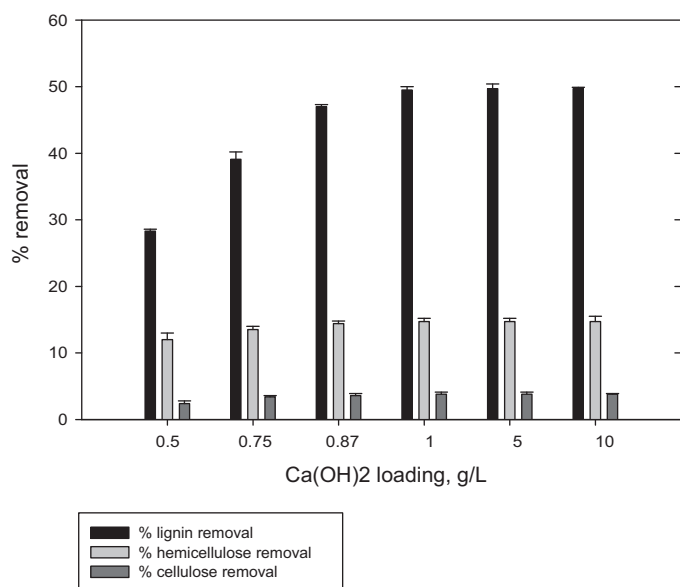
Fig. 2. Screening the effects of the \text{Ca}(\text{OH})_2 concentration on delignification.
